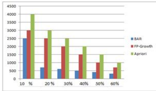
Fig.3: Comparative Analysis of Rule Generation
