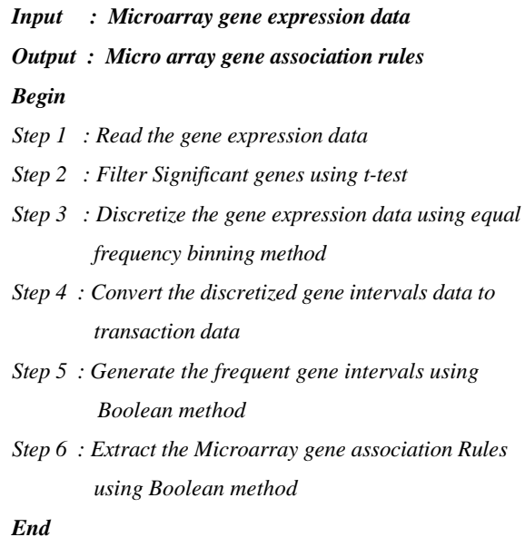
Fig.2: BAR Algorithm
